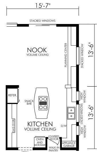
OPTIONAL KITCHEN
