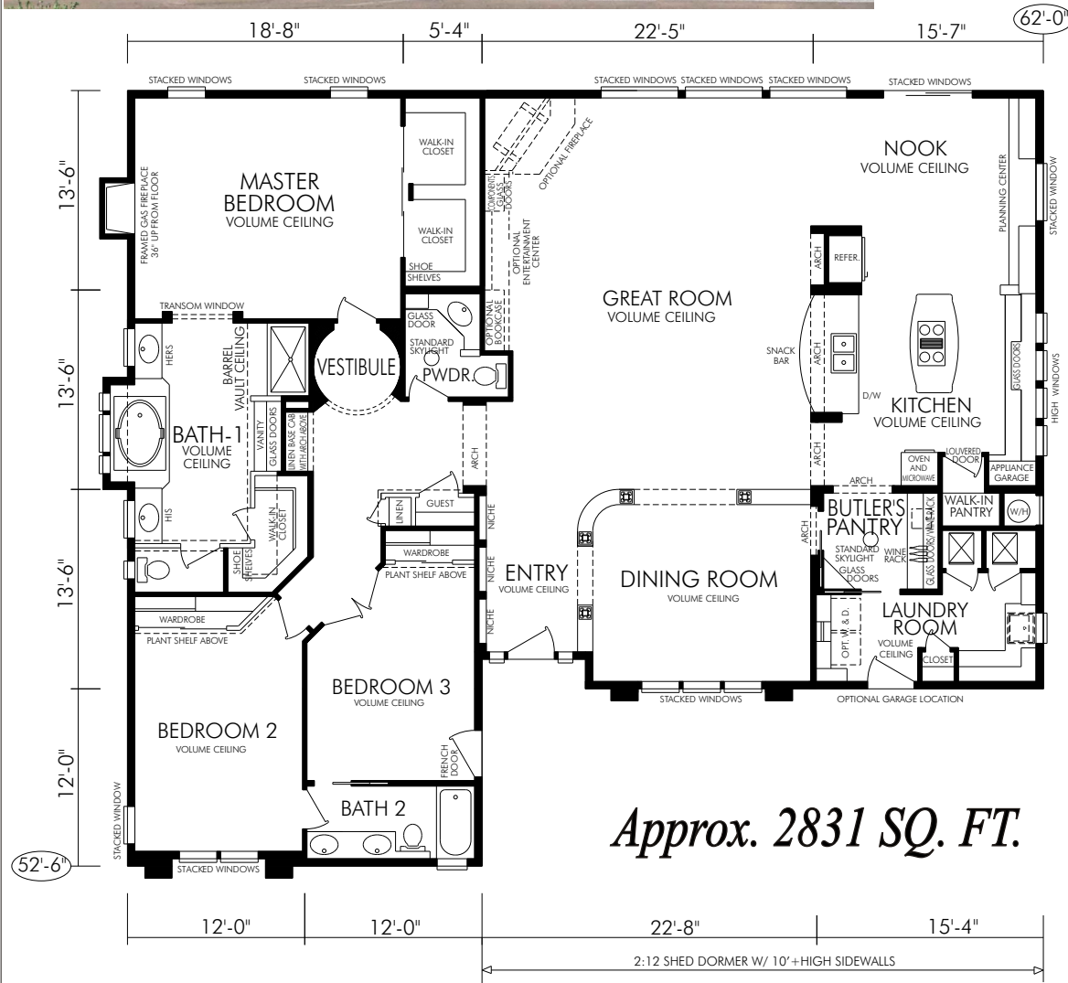
OPTIONAL KITCHEN
